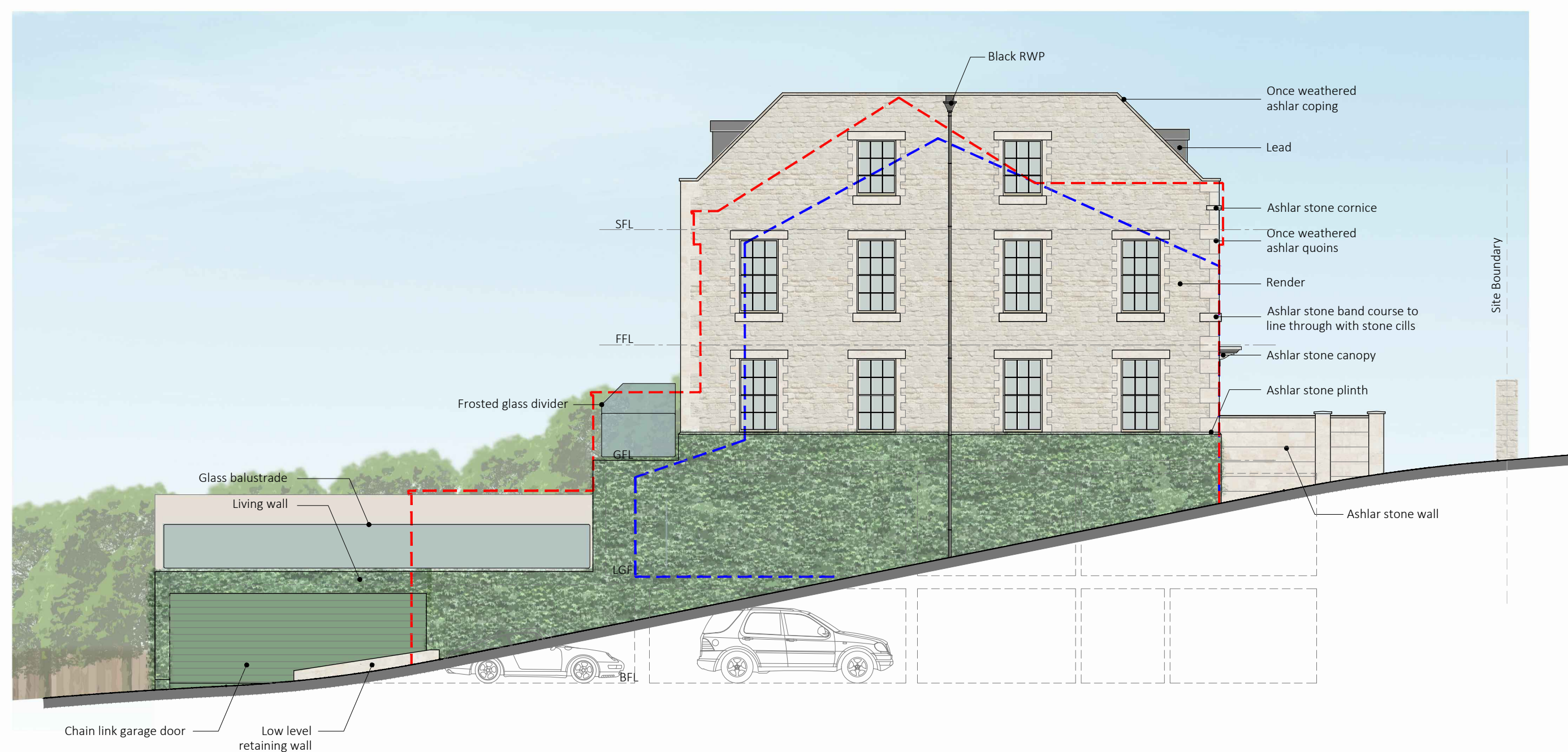
SIDE ELEVATION
