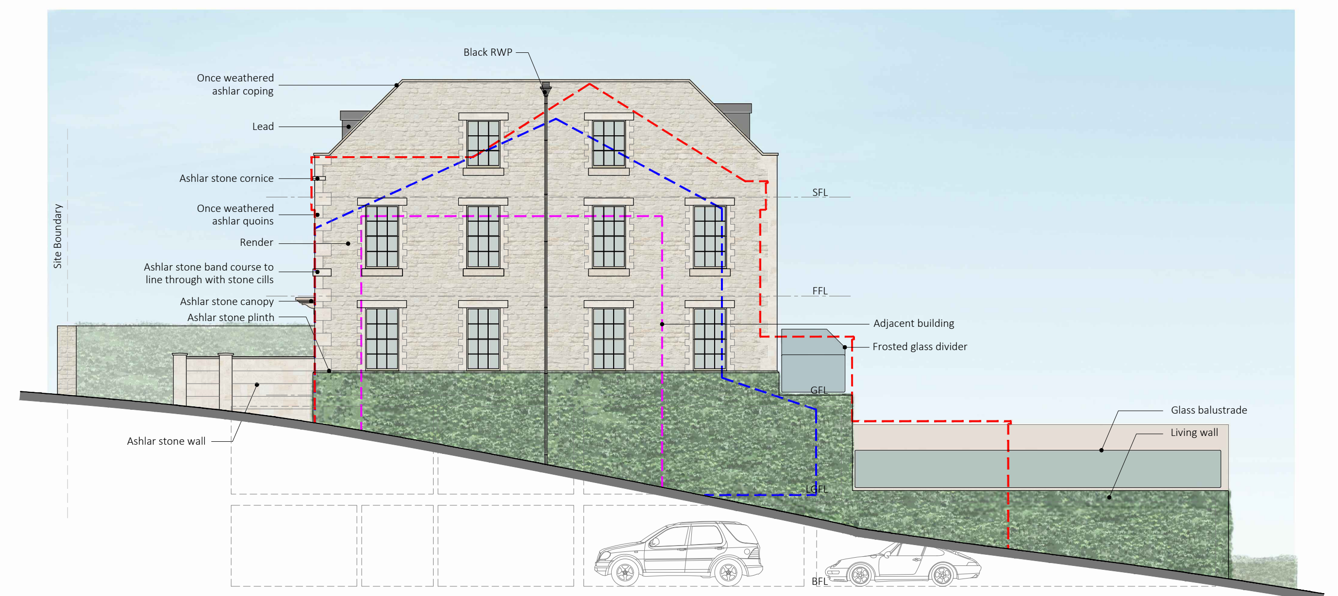
SIDE ELEVATION
